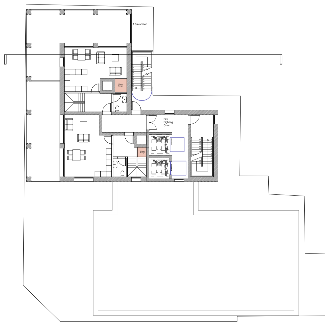
Proposed Floor Plan 08 - 1:200 0 2 4 6 8 10
